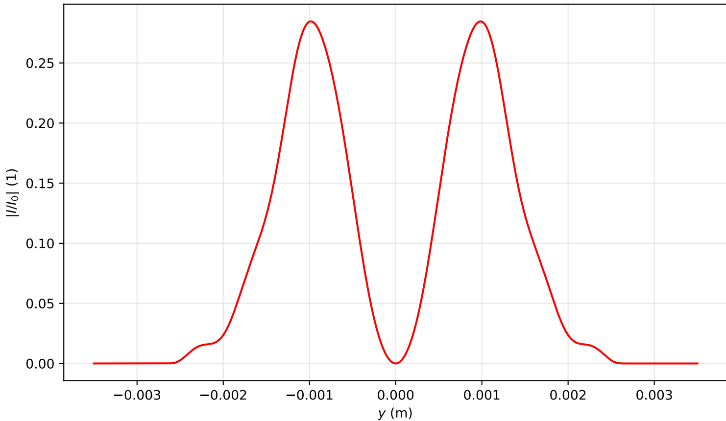
Intensity profile I(x=0, y, z=3.742)/I_0 , P_{in}=2.0P_{cr} , artificial time
